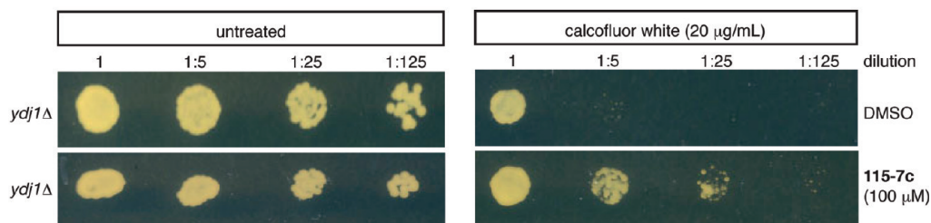
Figure 2. Compound 115-7c partially circumvents loss-of-function mutations in the J-domain containing co-chaperone, Ydj1, in yeast. A Addition of 115-7c (100 \mu\text{M} ), but not the solvent control, partially restores growth at elevated temperatures in a ydj1 Δ strain. B Deletion of Ydj1 sensitizes cells to treatment with calcofluor white, and application of 115-7c (100 \mu\text{M} ) partially suppresses this phenotype.
