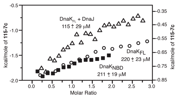
(A) 115-7c binds to both DnaK and the DnaK-DnaJ complex
