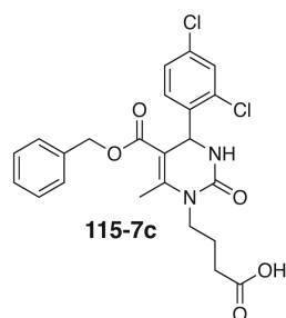
(A) Chemical structure of 115-7c
