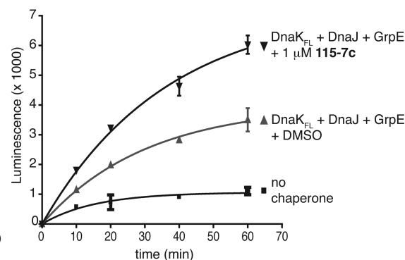
Figure 1. Compound 115-7c stimulates the ATPase and folding activities of Hsp70-family chaperones. A) Chemical structure of the dihydropyrimidine, 115-7c. B) 115-7c promotes the ATPase activity of E. coli DnaK (DnaK FL ) and a truncated DnaK containing only the nucleotide-binding domain (DnaK NBD ). Results are the average of triplicates, and the error bars represent the standard deviations. The concentration of proteins: DnaK (0.6 μM), DnaJ (1.0 μM), GrpE (0.9 μM). C) 115-7c promotes the luciferase-folding activity of the DnaK FL -DnaJ-GrpE complex. Results are the average of triplicates and the error bars represent the standard deviations. The concentration of proteins: DnaK (0.2 μM), DnaJ (0.05 μM), GrpE (0.02 μM).
