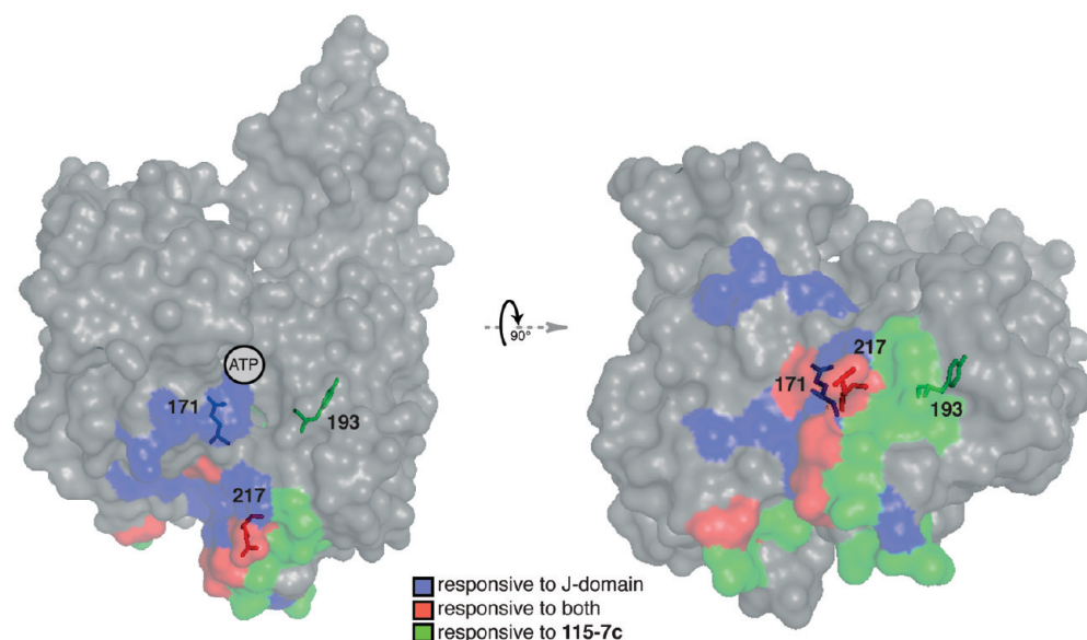
(B) Mutations in DnaK suggest non-overlapping allosteric pathways
