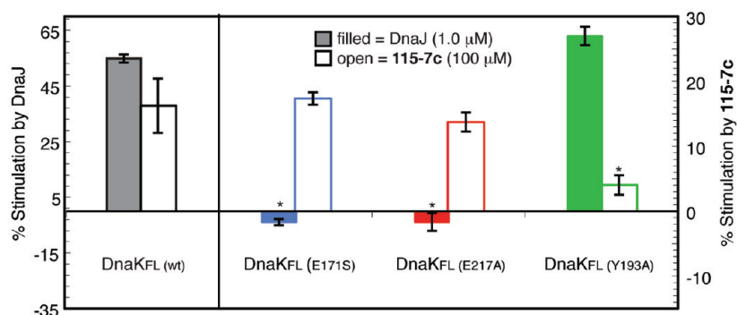
Figure 4. Site-directed mutagenesis suggests at least two allosteric pathways that stimulate the ATPase activity of DnaK. A) Overlay of the residues identified by NMR as responsive to 115-7c (green), those known to be important for J-domain activity (purple), and those amino acids that fit in both categories (red). The J-domain responsive residues were assembled from published studies in which point mutants in Hsp70s were found to block J-domain-mediated stimulation (17, 18, 42, 43). Two views are shown to highlight the fact that some of the responsive residues, such as E171 and Y193, are found in the protein interior, whereas others, such as E217, are surface residues. The overlay was generated in PyMol. B) Point mutants were generated in DnaK FL at either E171S, E217A, or Y193A. The Y193A mutation blocked 115-7c -mediated stimulation but did not completely prevent J-domain activity ( p < 0.0001 ), whereas the other mutations blocked stimulation by DnaJ. Results are the average of (at least) triplicates and error bars represent the standard deviations.
